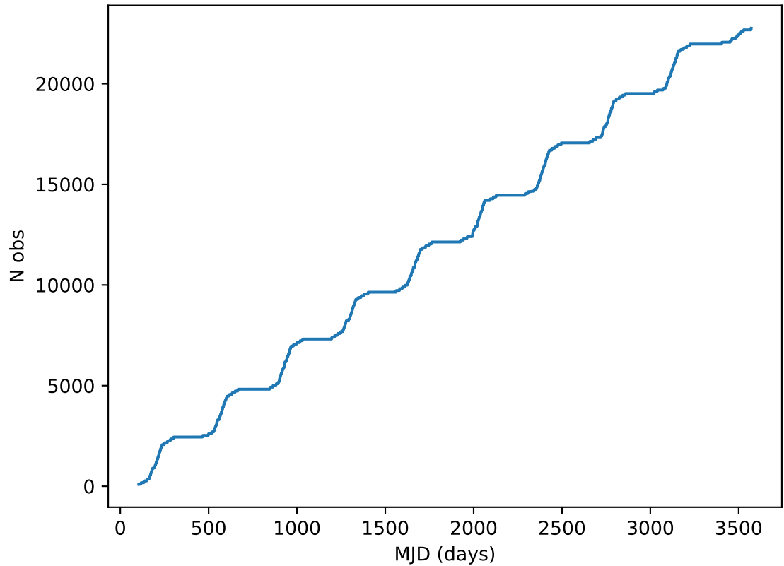
ddf_acor_sf20_lsf40_lsr20_v3.4_10yrs all bands: DD:ECDFS Cumulative NVisits
