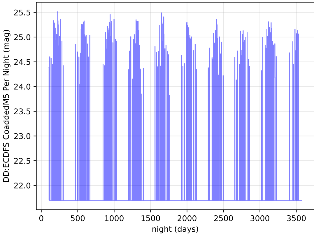
ddf_acor_sf20_lsf40_lsr20_v3.4_10yrs z band: DD:ECDFS CoaddedM5 Per Night
