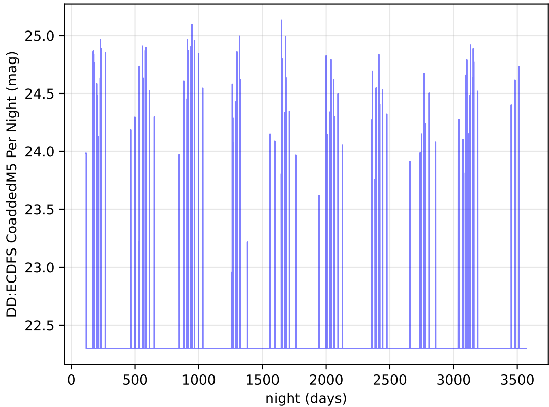
ddf_acor_sf20_lsf40_lsr20_v3.4_10yrs u band: DD:ECDFS CoaddedM5 Per Night
