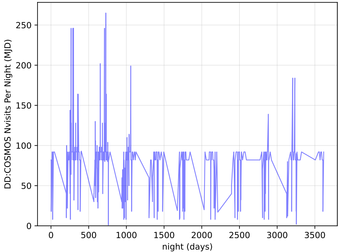
ddf_acor_sf20_lsf40_lsr20_v3.4_10yrs all bands: DD: COSMOS Nvisits Per Night
