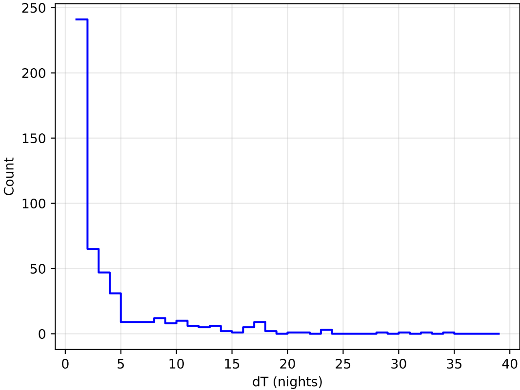
ddf_acor_sf20_Isf40_Isr20_v3.4_10yrs all bands: DD: COSMOS Delta Nights Histogram
