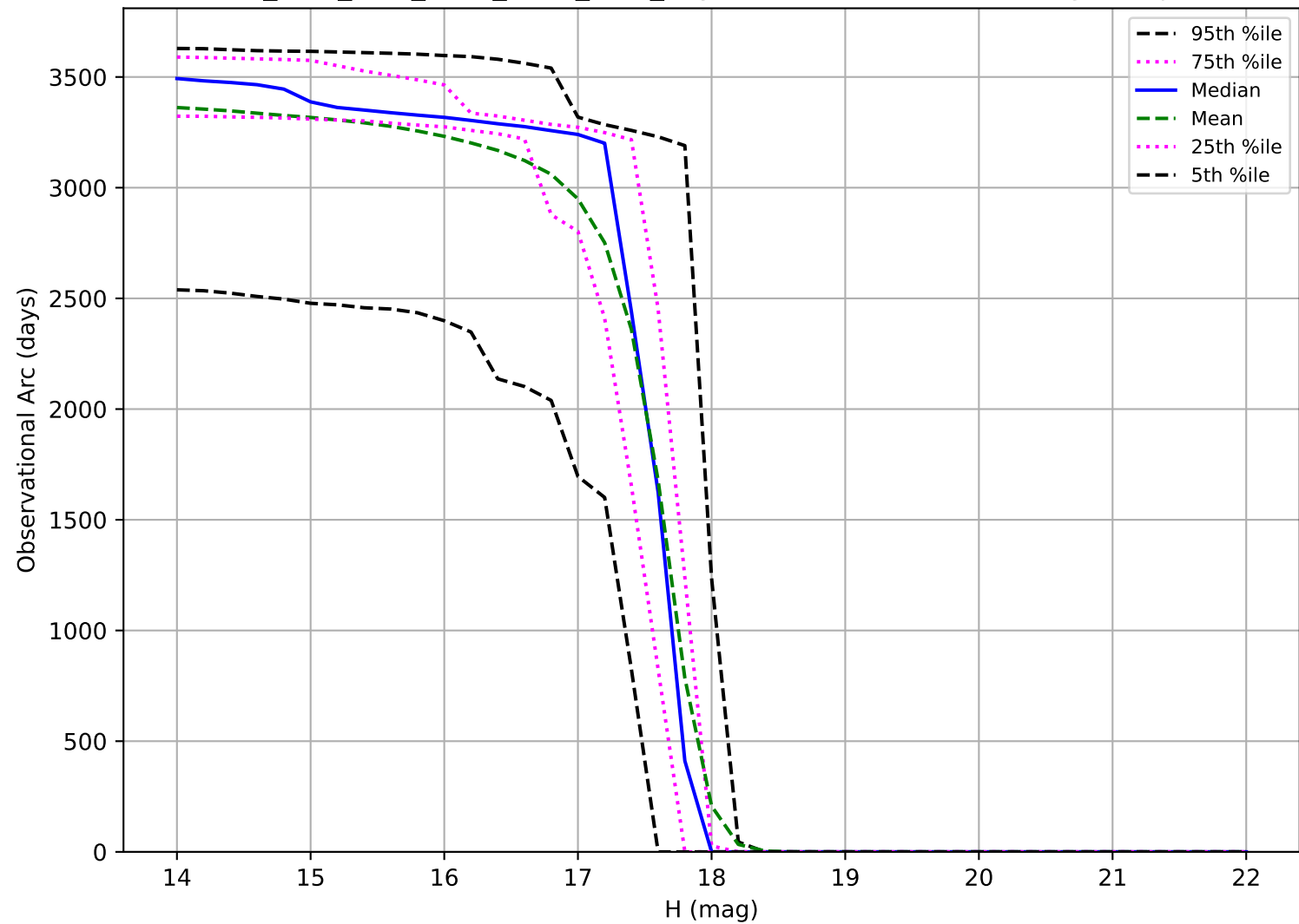
ddf_acor_sf20_lsf40_lsr10_v3.4_10yrs: Observational Arc Length Trojan
