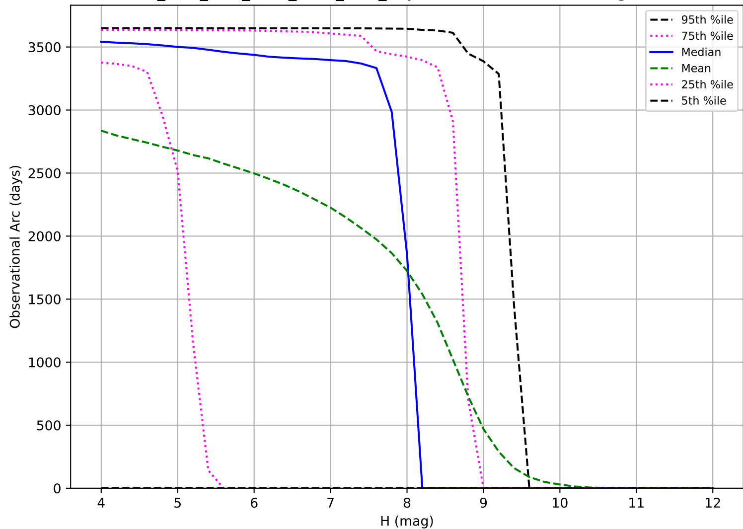
ddf_acor_sf20_Isf40_Isr10_v3.4_10yrs: Observational Arc Length TNO
