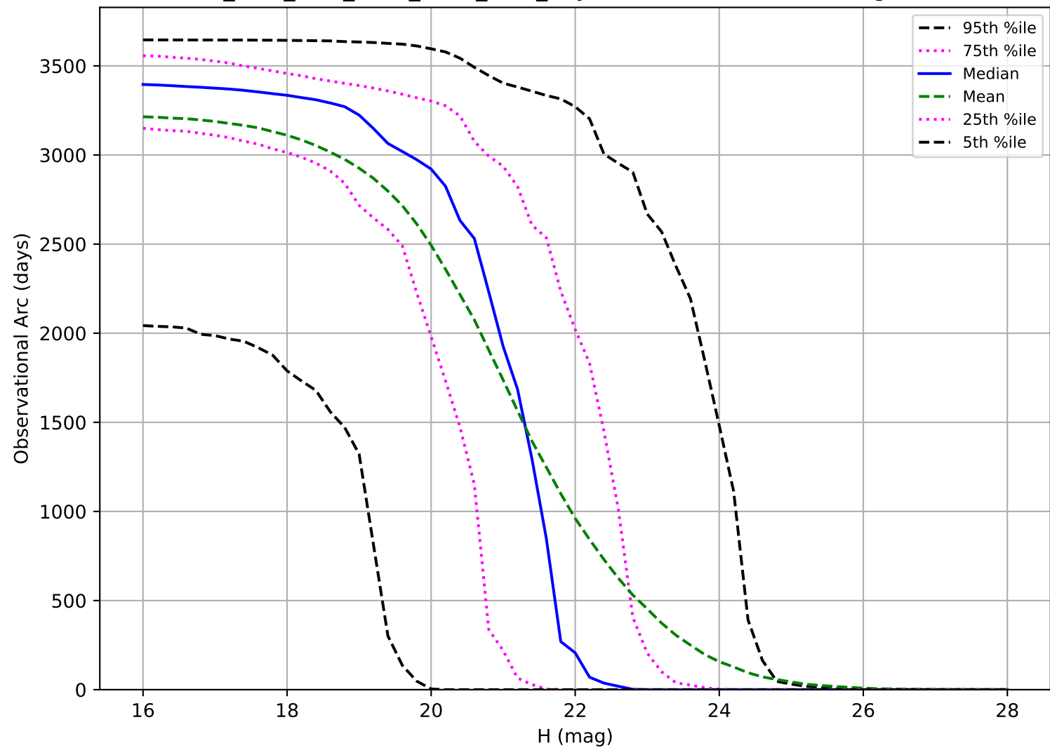
ddf_acor_sf20_lsf40_lsr10_v3.4_10yrs: Observational Arc Length PHA
