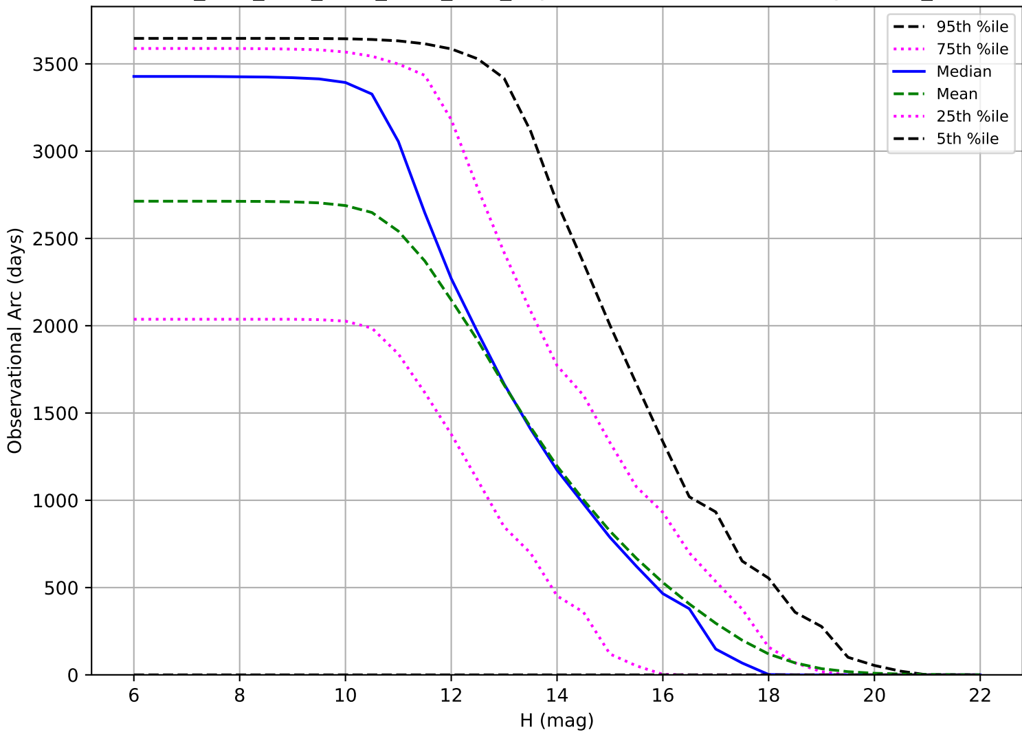
ddf_acor_sf20_lsf40_lsr10_v3.4_10yrs: Observational Arc Length OCC_r5
