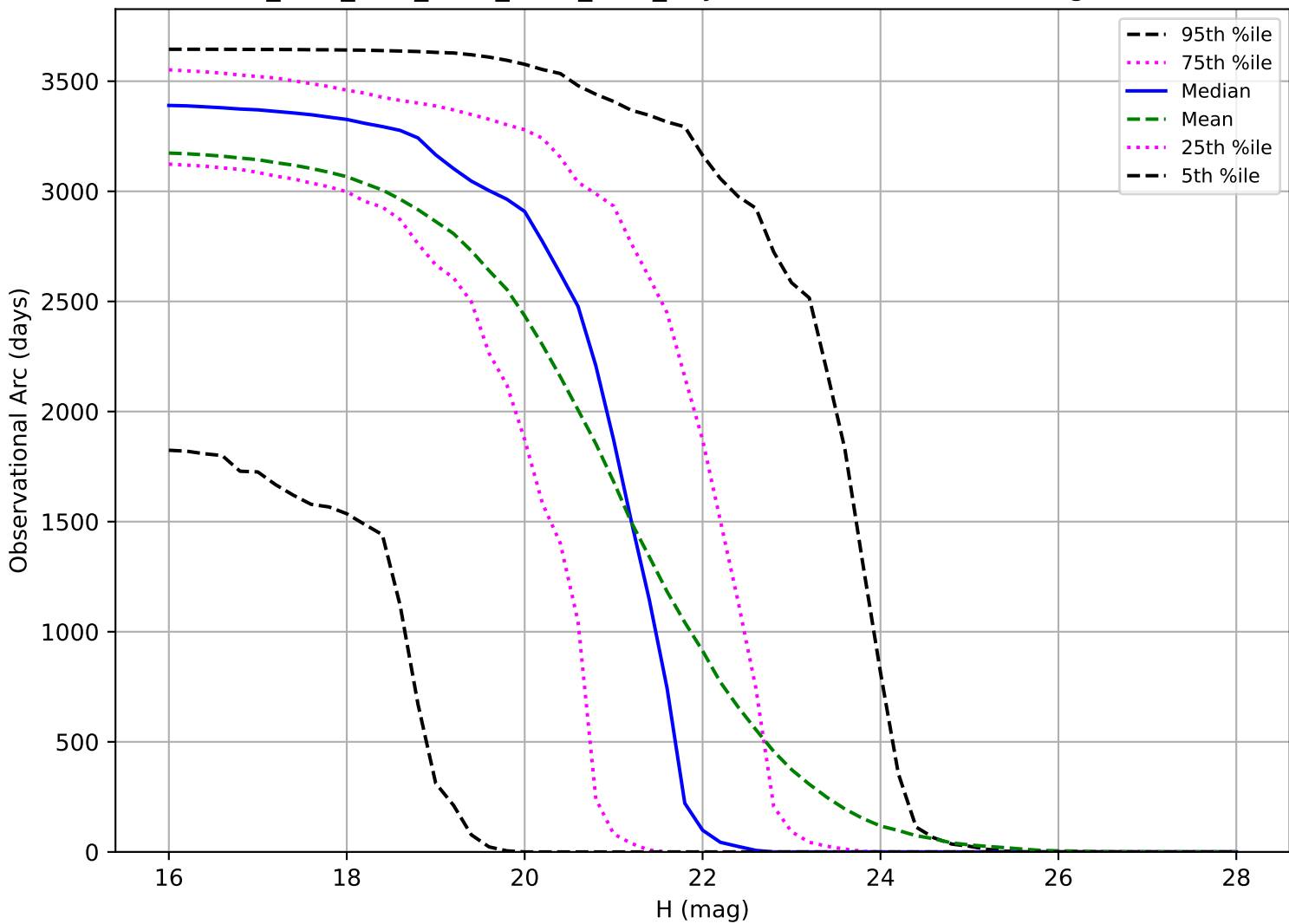
ddf_acor_sf20_lsf40_lsr10_v3.4_10yrs: Observational Arc Length NEO
