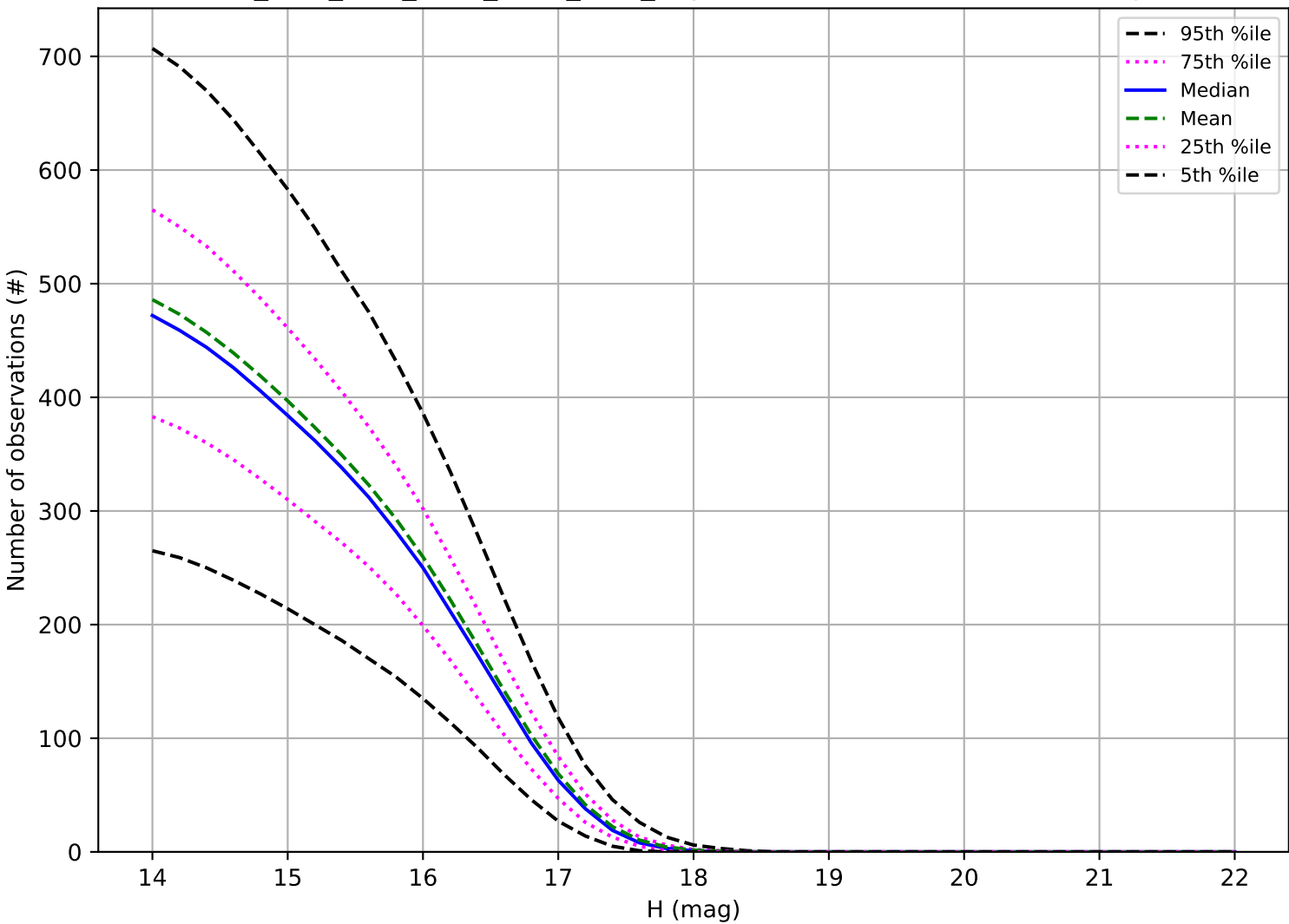
ddf_acor_sf20_lsf40_lsr10_v3.4_10yrs: Number of observations Trojan
