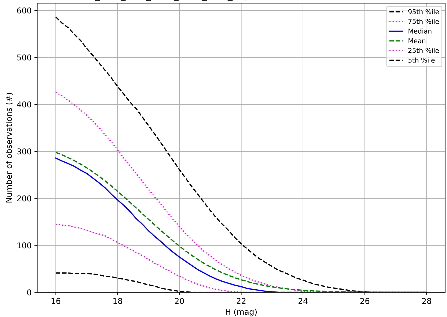
ddf_acor_sf20_lsf40_lsr10_v3.4_10yrs: Number of observations PHA
