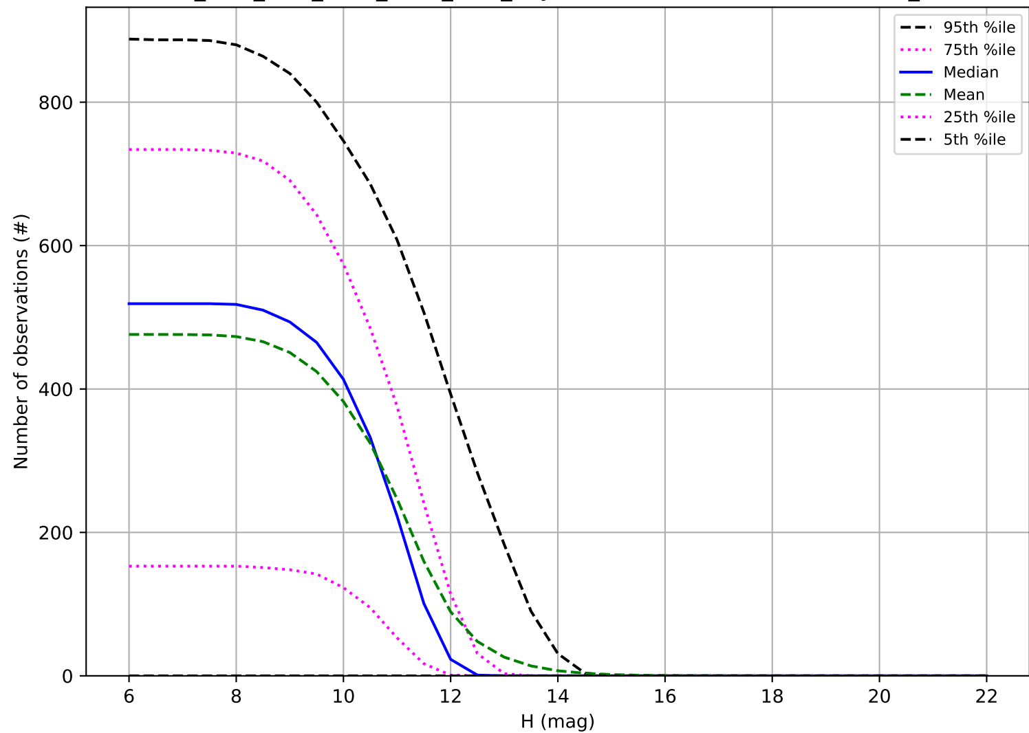
ddf_acor_sf20_lsf40_lsr10_v3.4_10yrs: Number of observations OCC_r20
