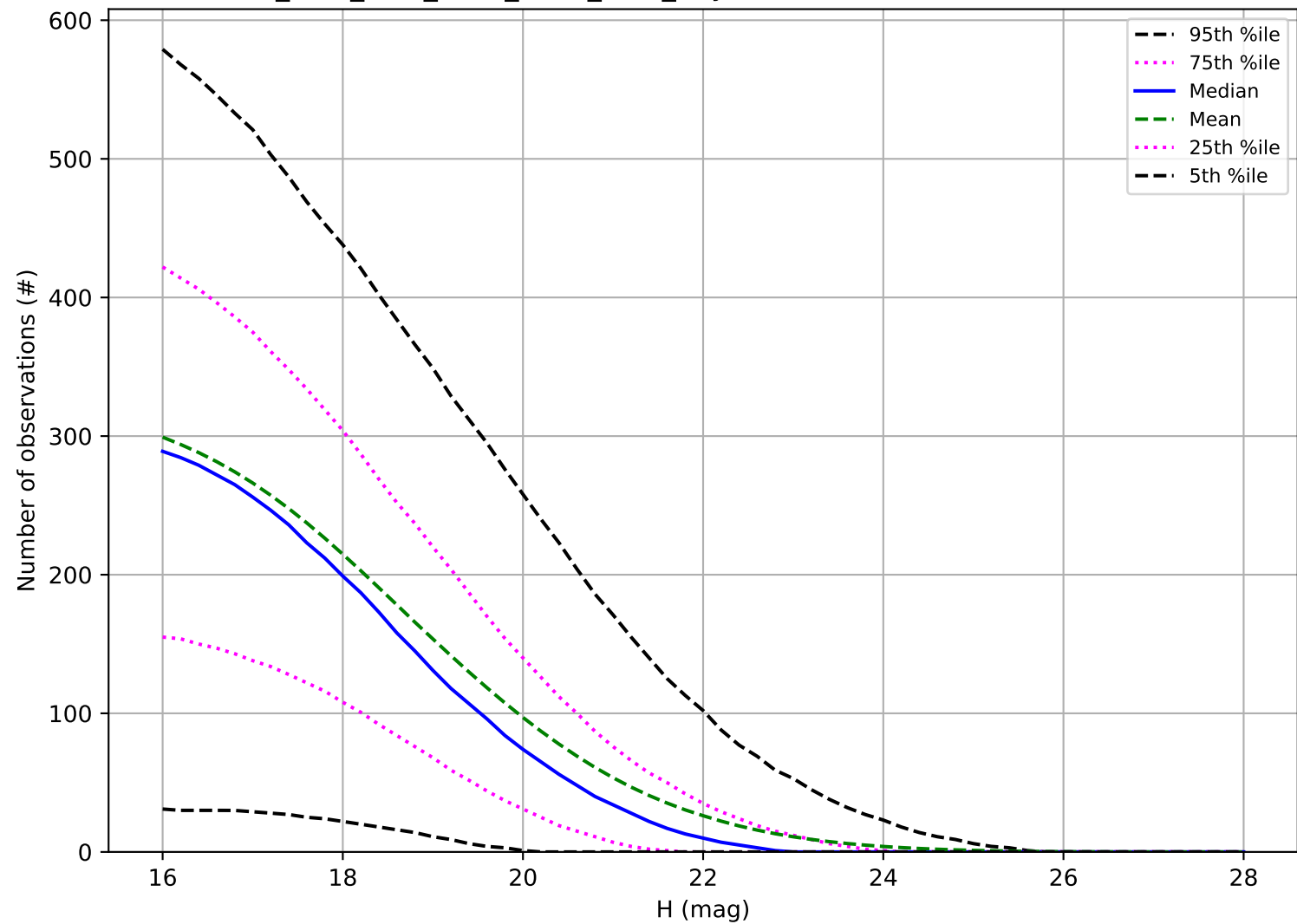
ddf_acor_sf20_lsf40_lsr10_v3.4_10yrs: Number of observations NEO
