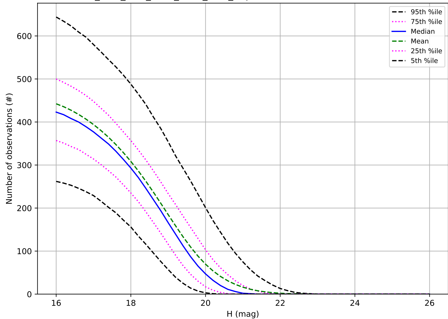
ddf_acor_sf20_lsf40_lsr10_v3.4_10yrs: Number of observations MBA
