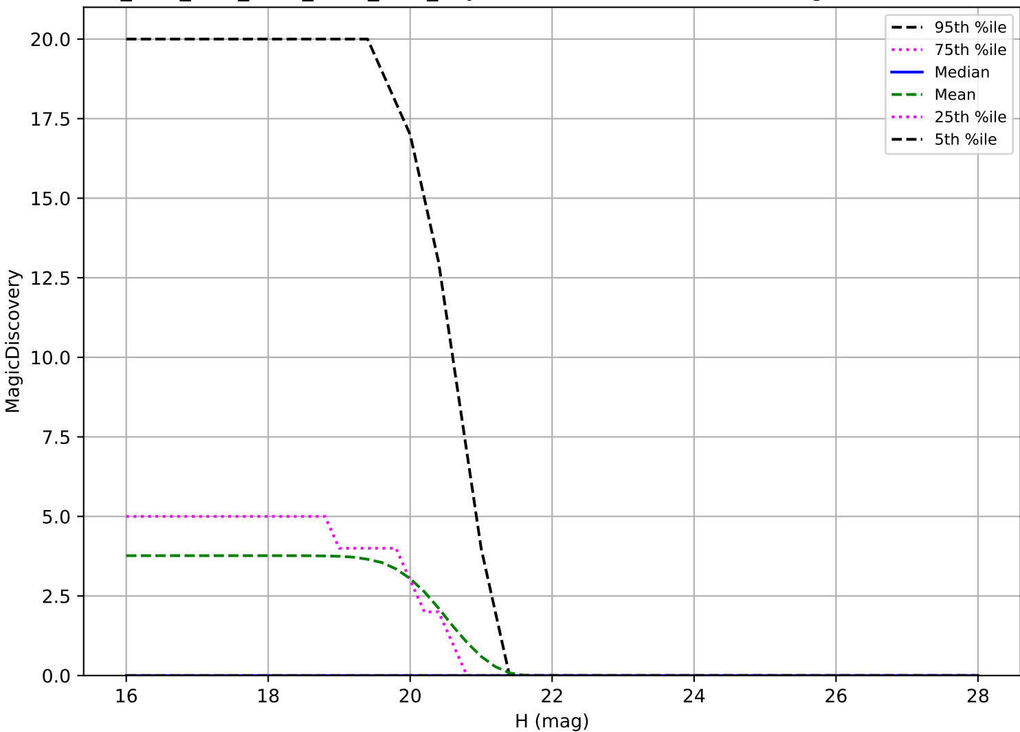
ddf_acor_sf20_lsf40_lsr10_v3.4_10yrs: Vatira 6 detections in 60 nights detection loss
