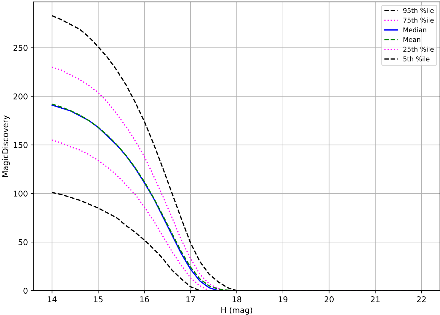
ddf_acor_sf20_lsf40_lsr10_v3.4_10yrs: Trojan 6 detections in 60 nights detection loss
