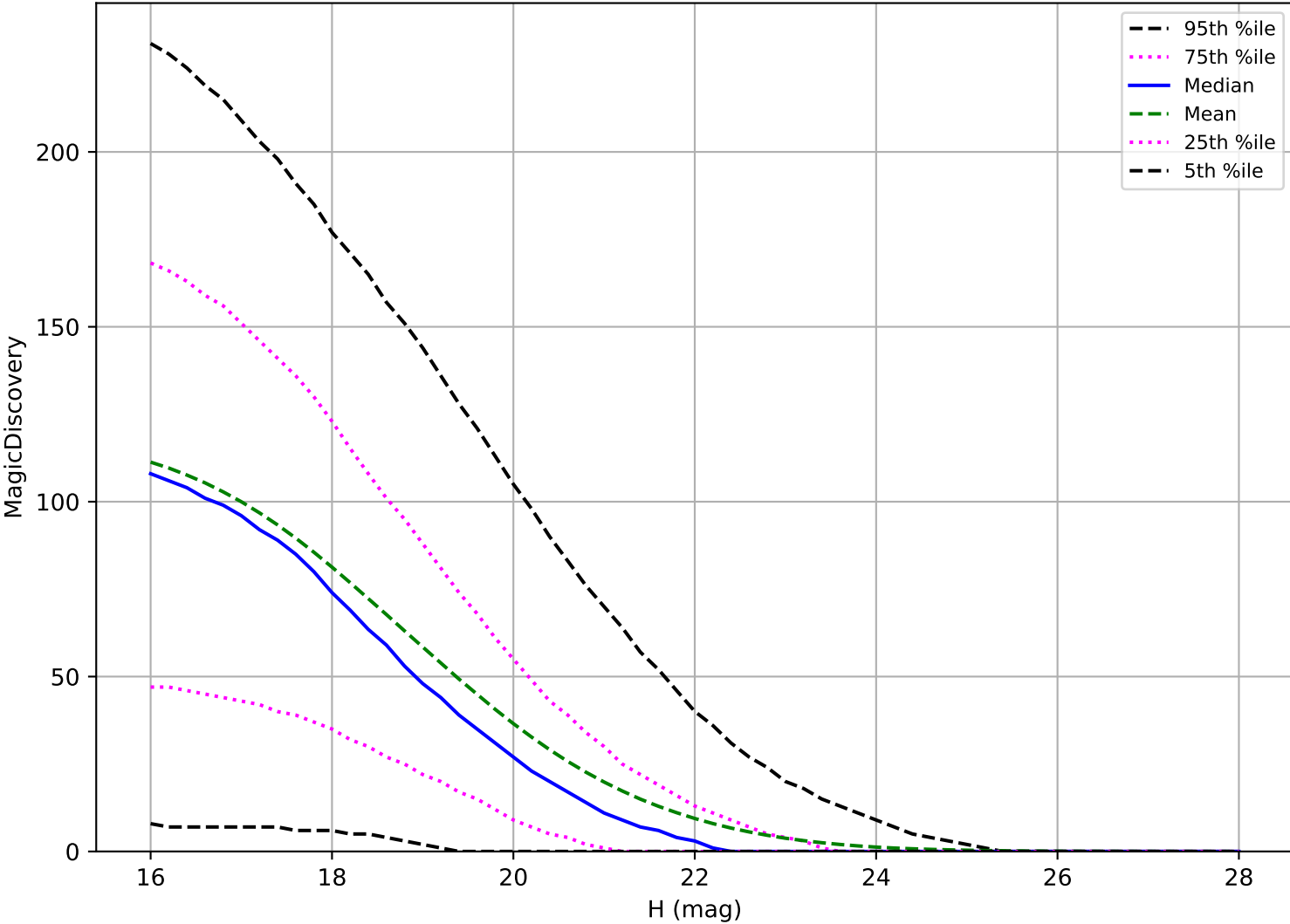
ddf_acor_sf20_lsf40_lsr10_v3.4_10yrs: PHA 6 detections in 60 nights detection loss
