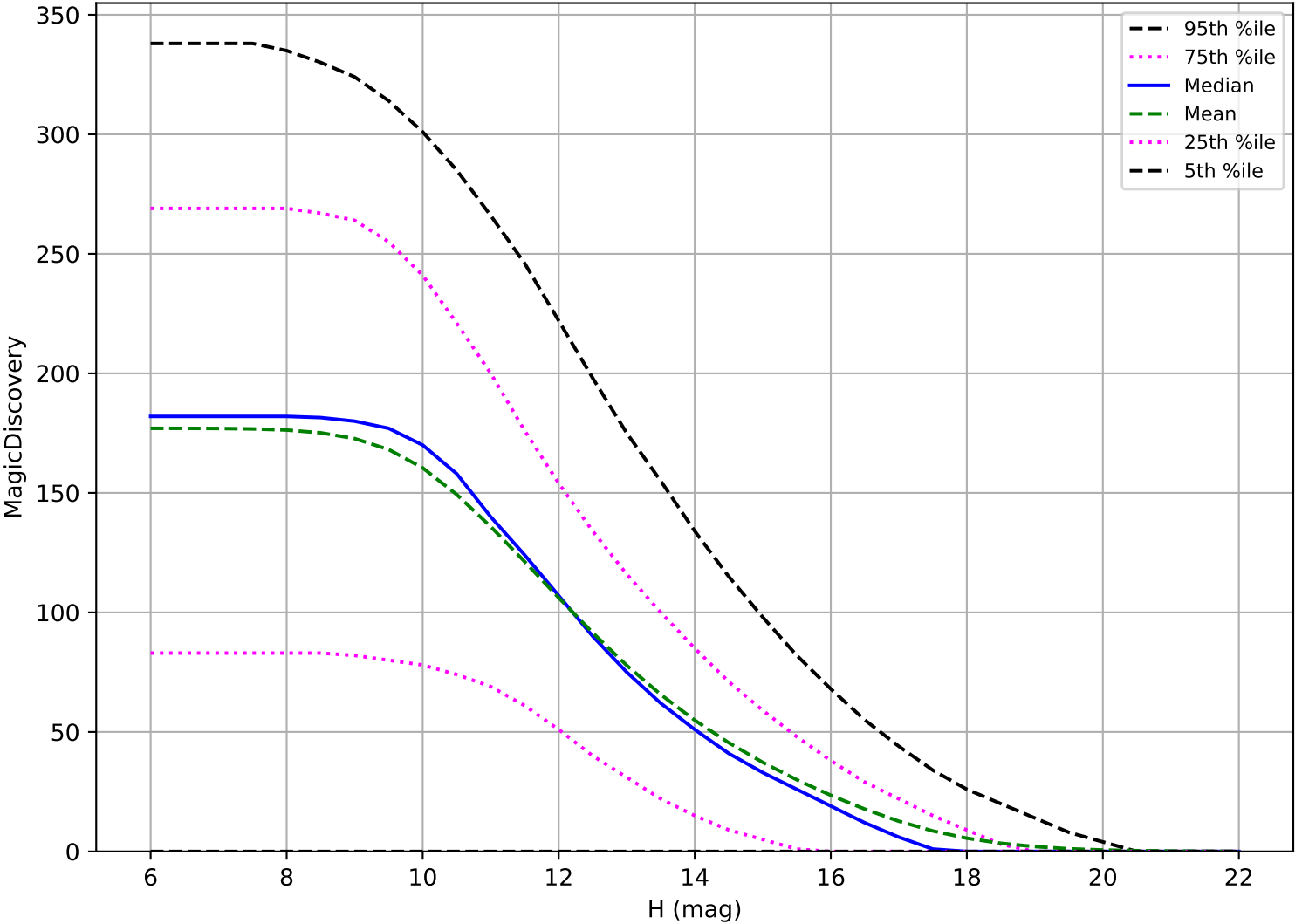
ddf_acor_sf20_lsf40_lsr10_v3.4_10yrs: OCC_r5 6 detections in 60 nights detection loss
