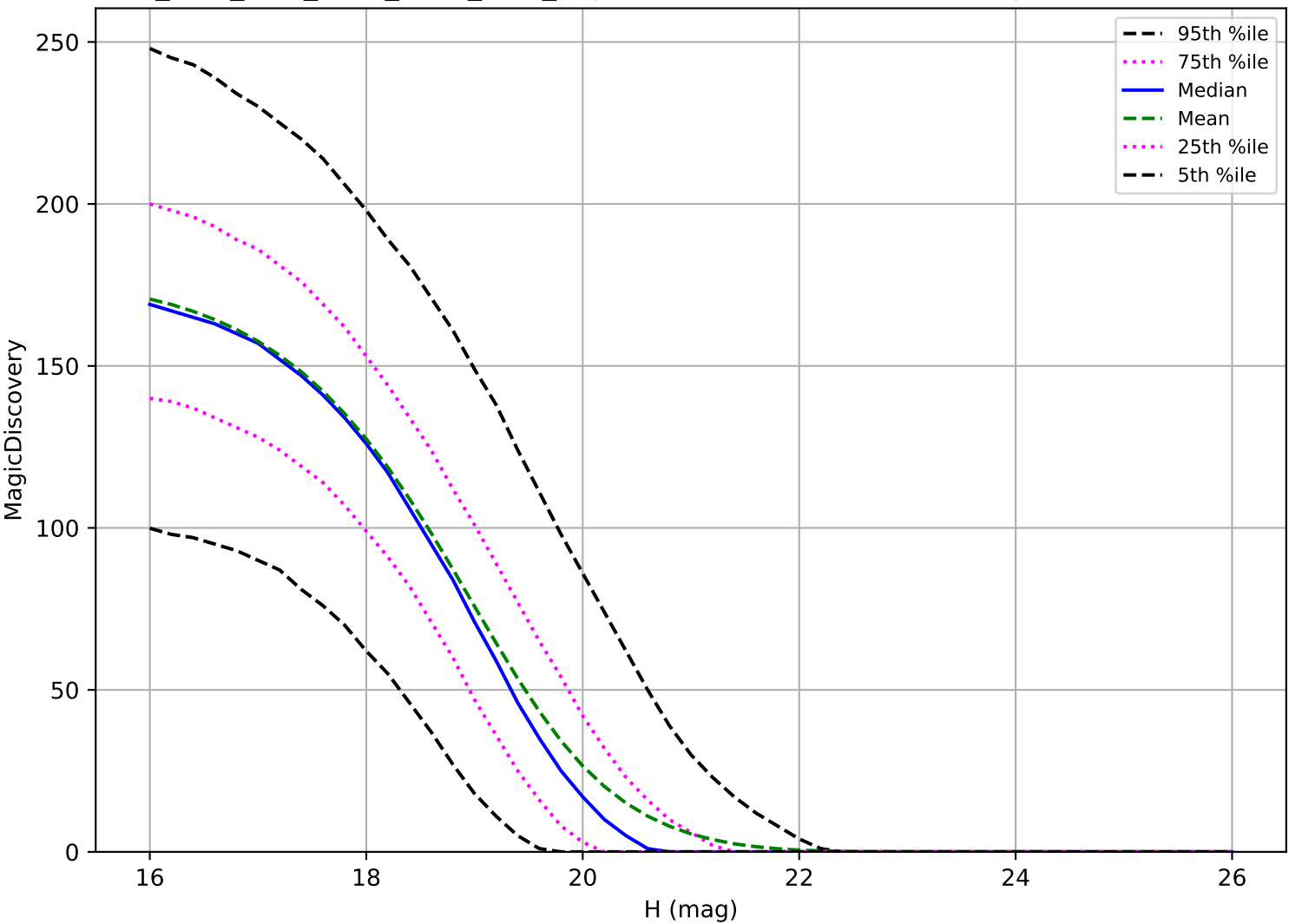
ddf_acor_sf20_lsf40_lsr10_v3.4_10yrs: MBA 6 detections in 60 nights detection loss
