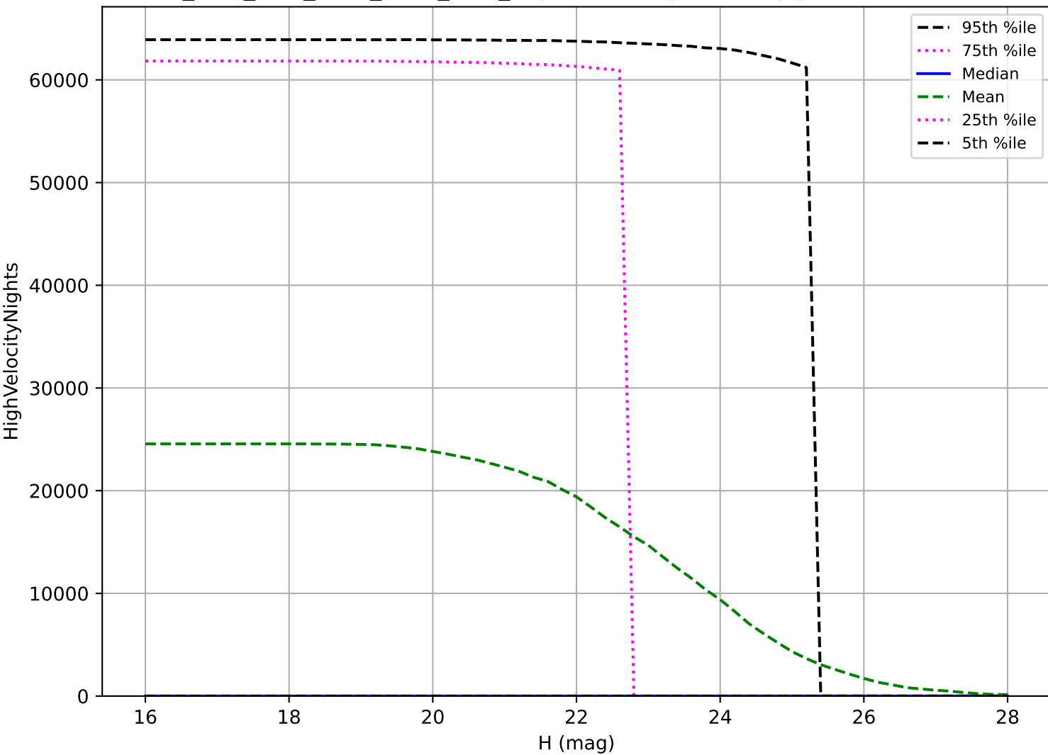
ddf_acor_sf20_lsf40_lsr10_v3.4_10yrs: PHA High velocity pair detection loss
