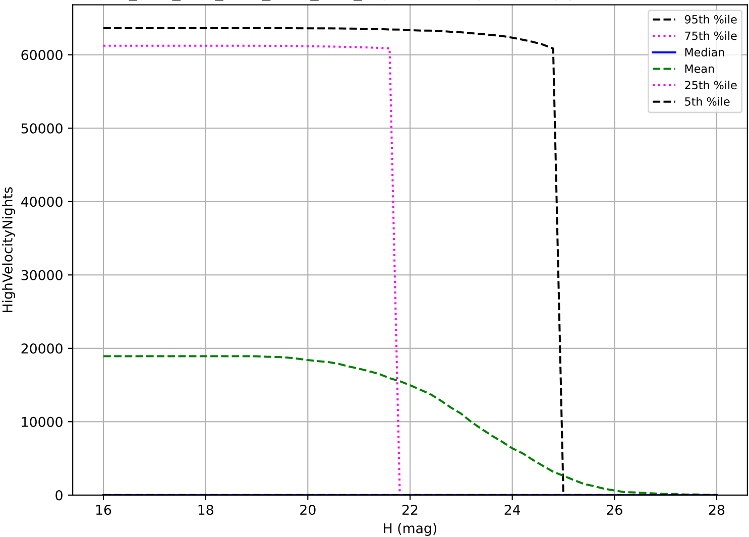
ddf_acor_sf20_lsf40_lsr10_v3.4_10yrs: NEO High velocity pair detection loss
