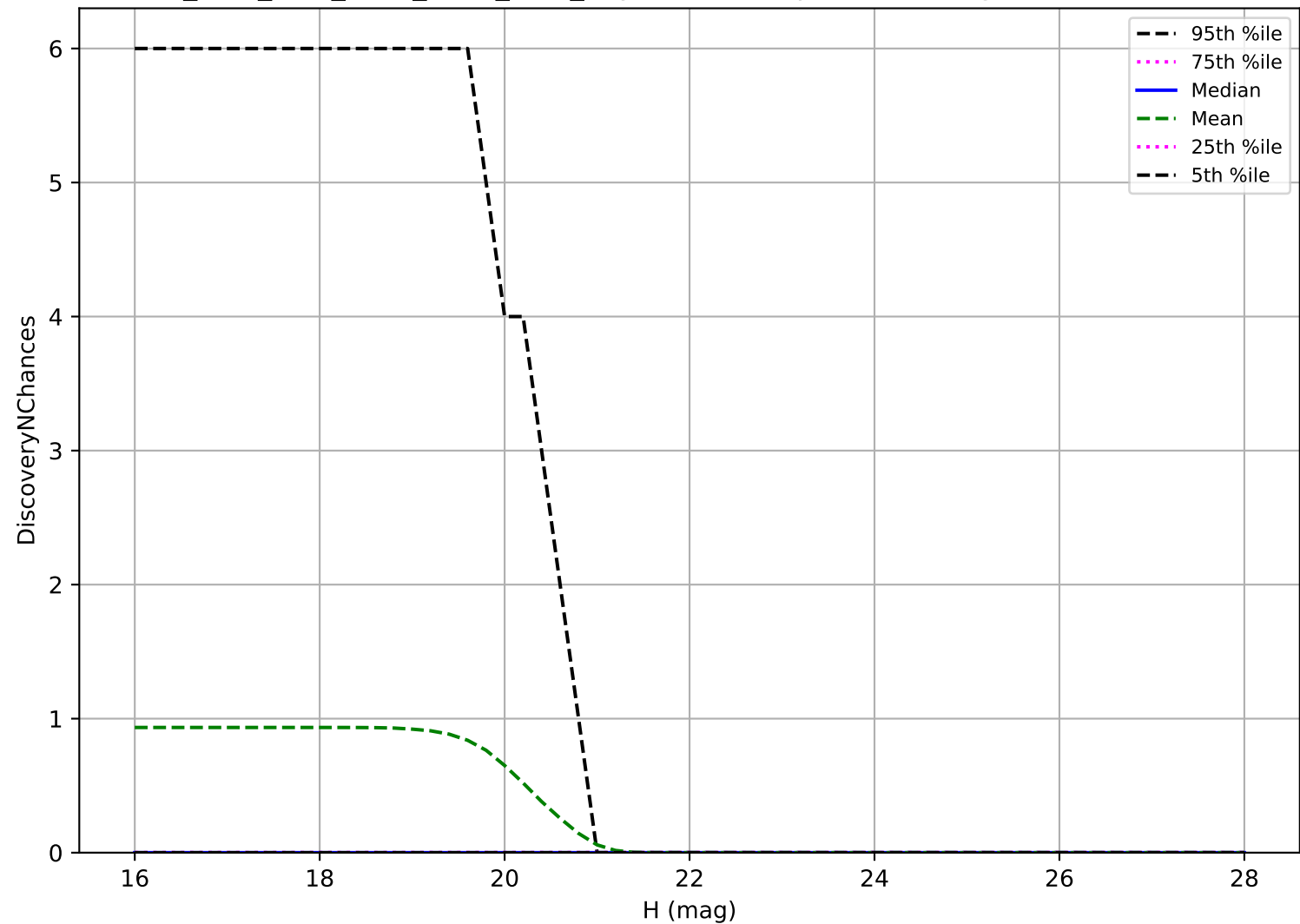
ddf_acor_sf20_lsf40_lsr10_v3.4_10yrs: Vatira 3 pairs in 15 nights detection loss
