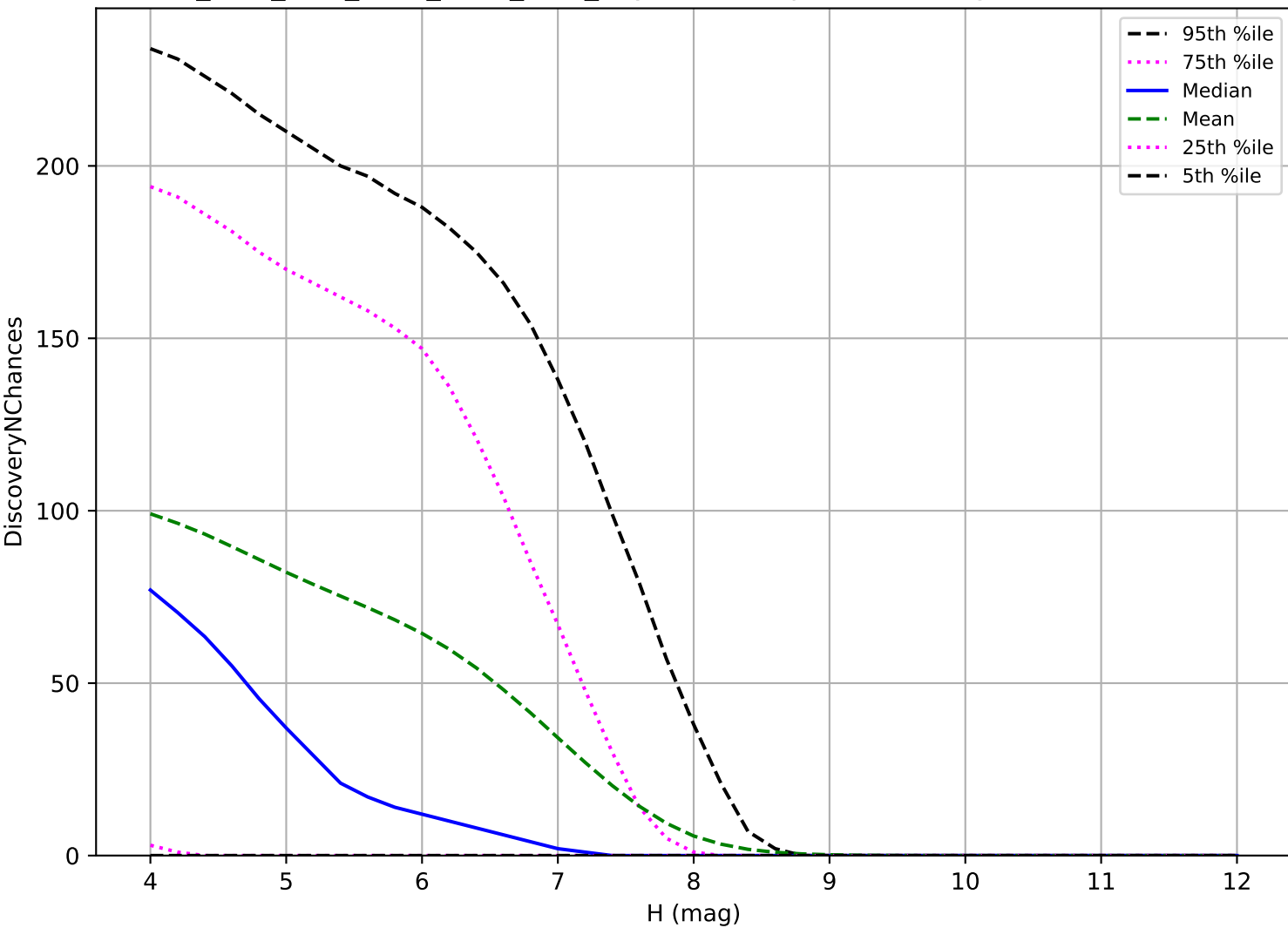
ddf_acor_sf20_lsf40_lsr10_v3.4_10yrs: TNO 3 pairs in 15 nights detection loss
