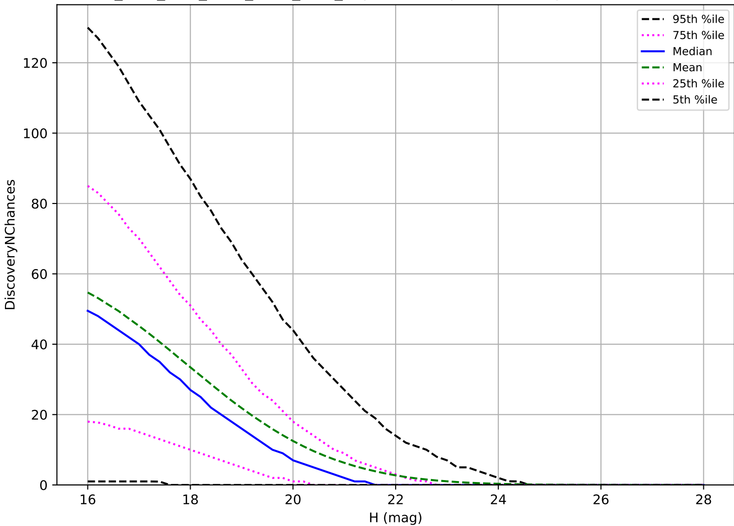
ddf_acor_sf20_lsf40_lsr10_v3.4_10yrs: PHA 3 pairs in 15 nights detection loss
