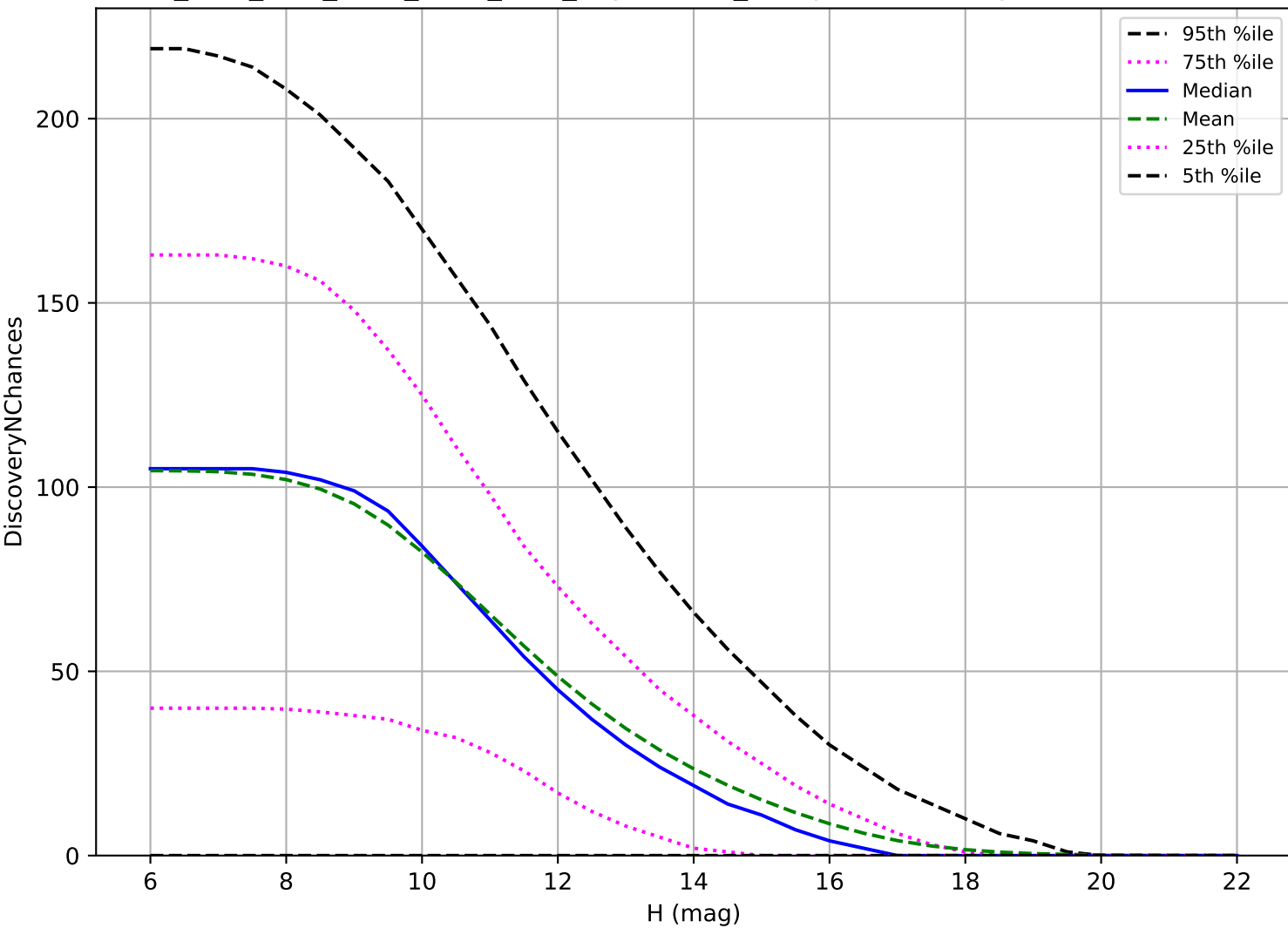
ddf_acor_sf20_lsf40_lsr10_v3.4_10yrs: OCC_r5 3 pairs in 15 nights detection loss
