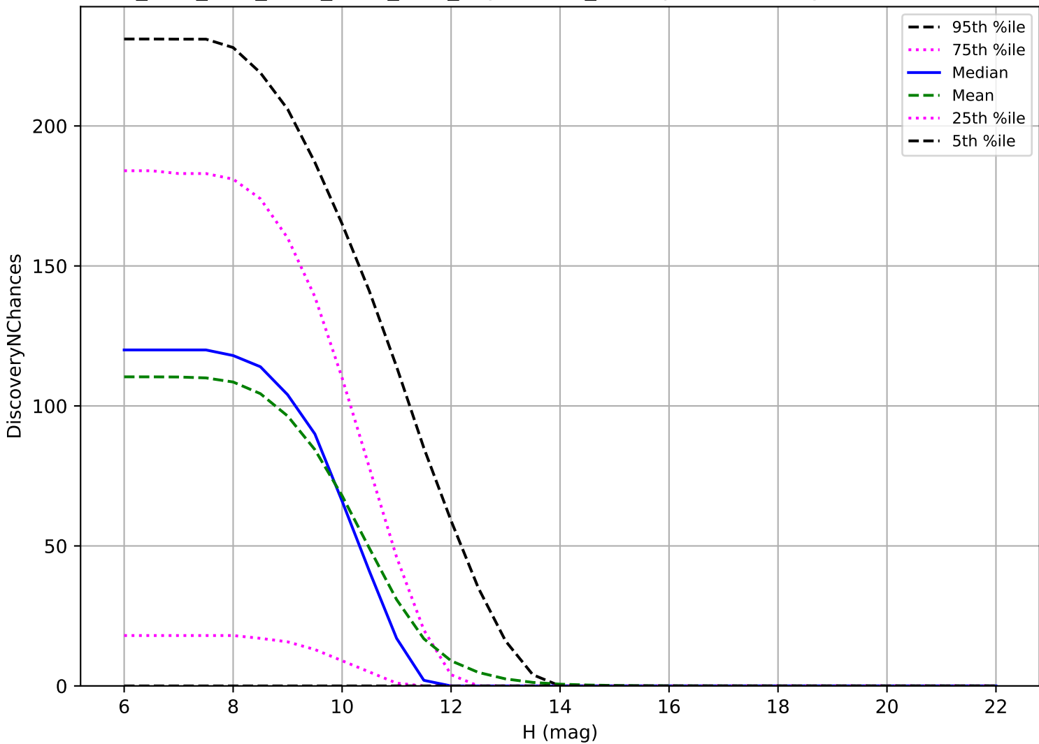
ddf_acor_sf20_lsf40_lsr10_v3.4_10yrs: OCC_r20 3 pairs in 15 nights detection loss
