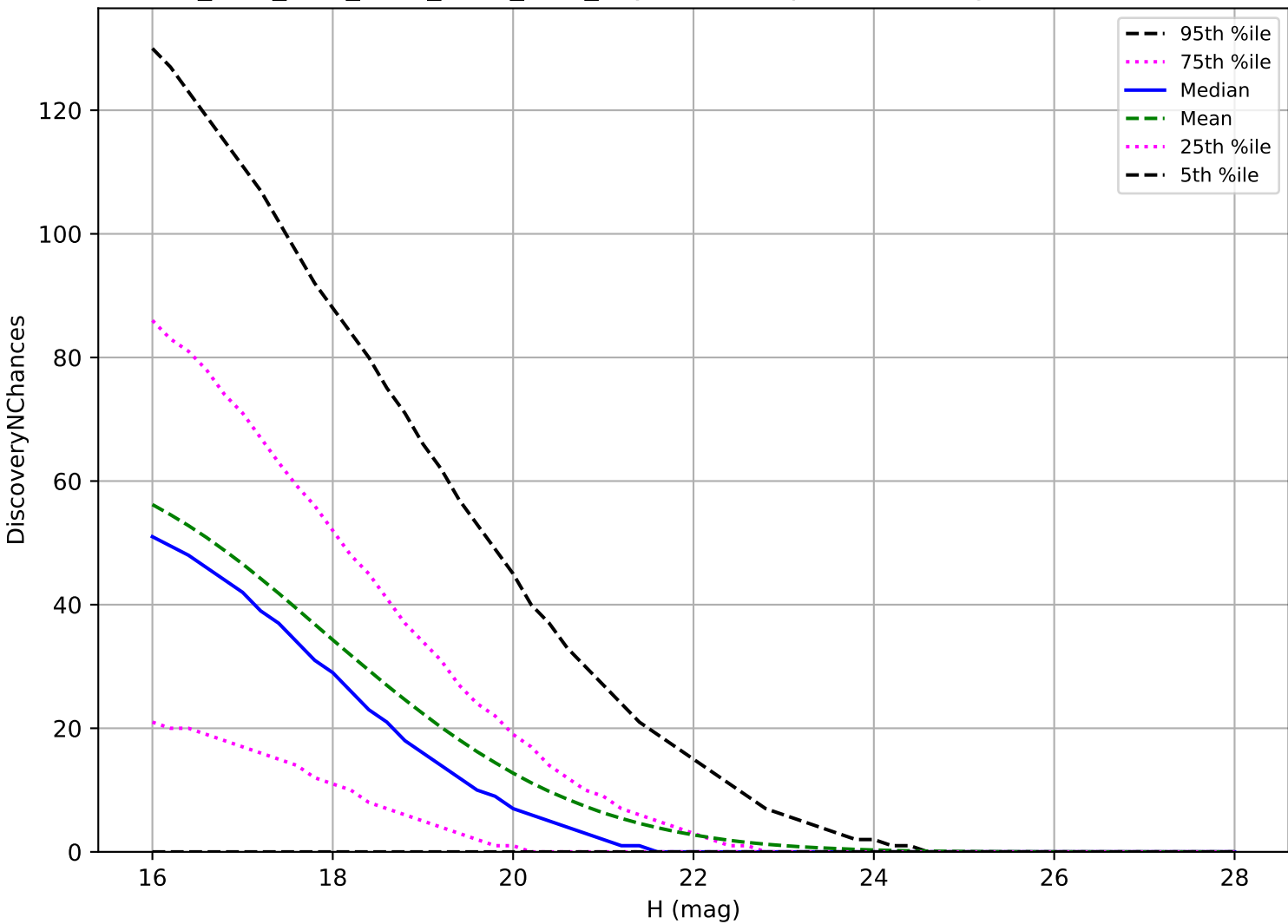
ddf_acor_sf20_lsf40_lsr10_v3.4_10yrs: NEO 3 pairs in 15 nights detection loss
