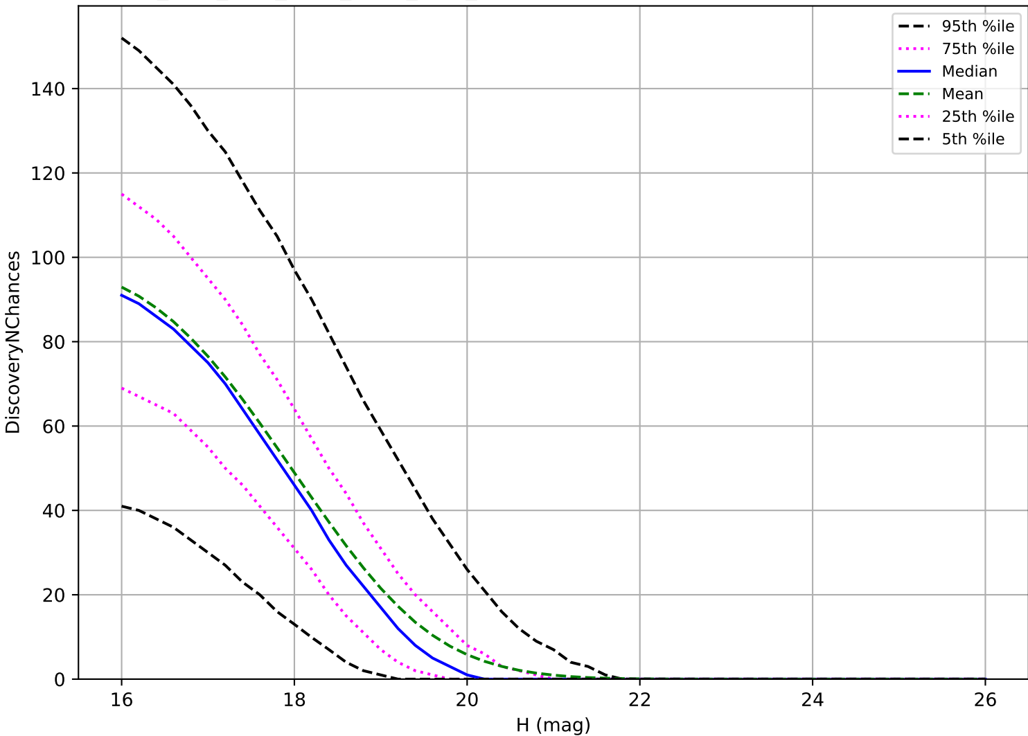
ddf_acor_sf20_lsf40_lsr10_v3.4_10yrs: MBA 3 pairs in 15 nights detection loss
