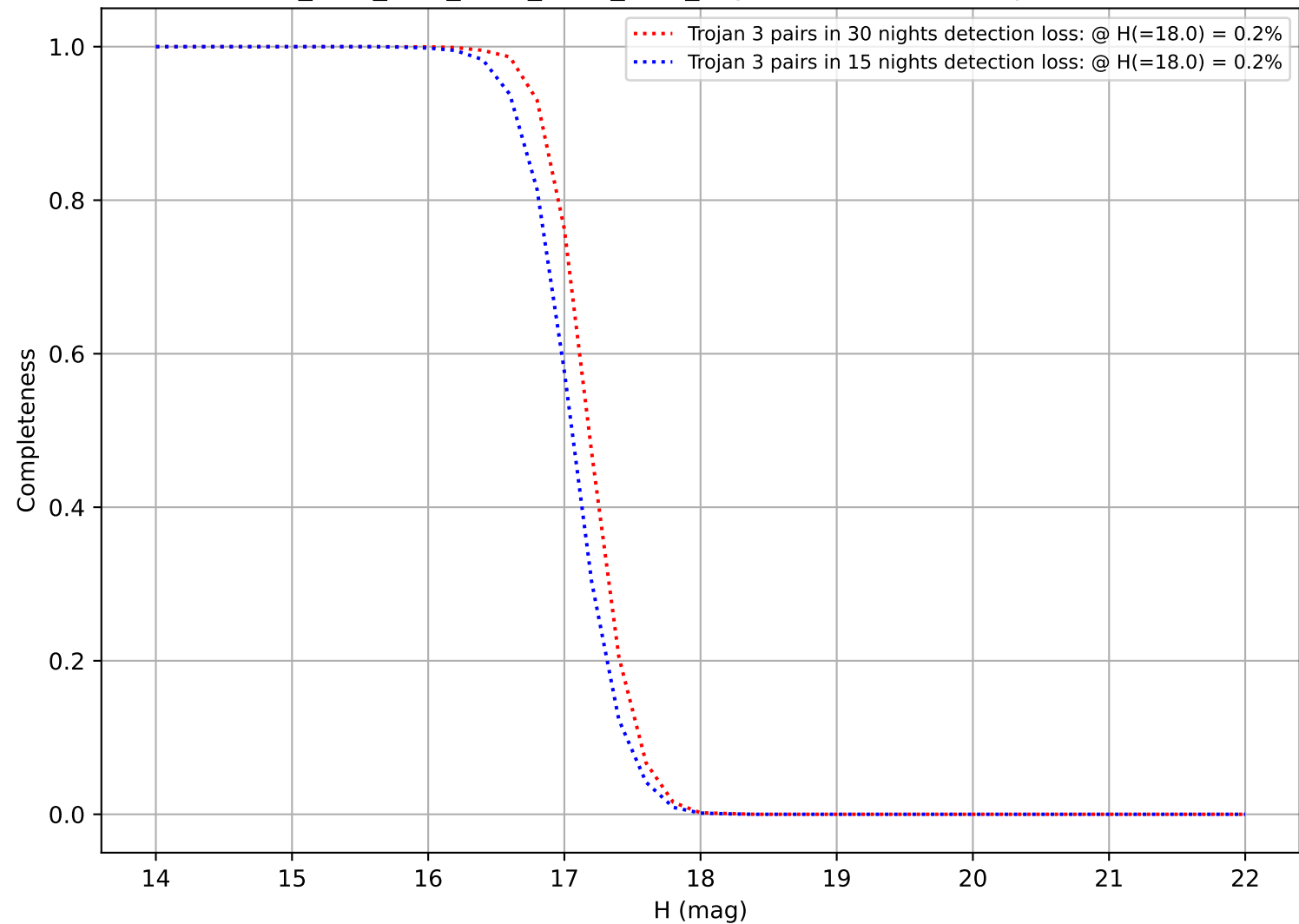
ddf_acor_sf20_lsf40_lsr10_v3.4_10yrs: DifferentialCompleteness
