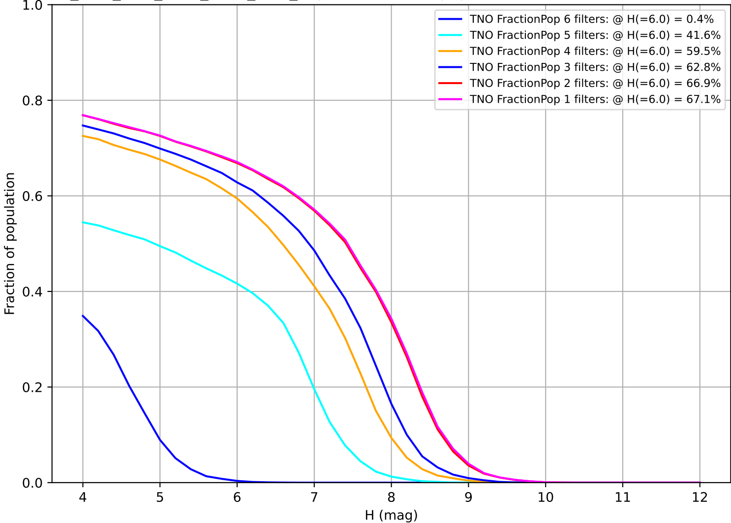
ddf_acor_sf20_lsf40_lsr10_v3.4_10yrs: Fraction of population with colors in X filters TNO
