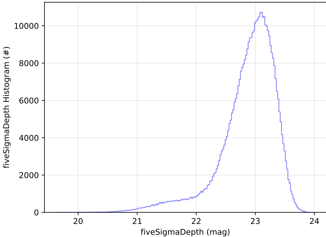
ddf_acor_sf20_lsf40_lsr10_v3.4_10yrs z: fiveSigmaDepth Histogram
