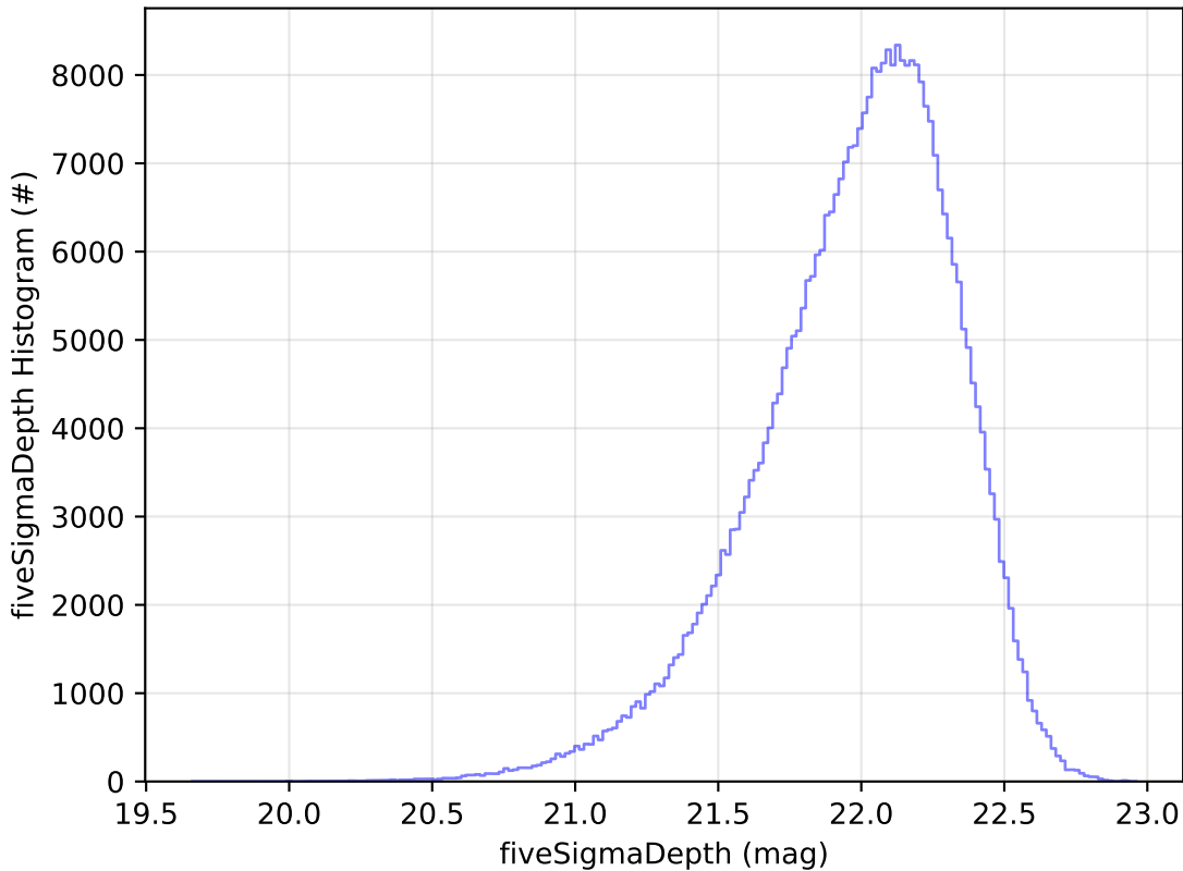
ddf_acor_sf20_lsf40_lsr10_v3.4_10yrs y: fiveSigmaDepth Histogram
