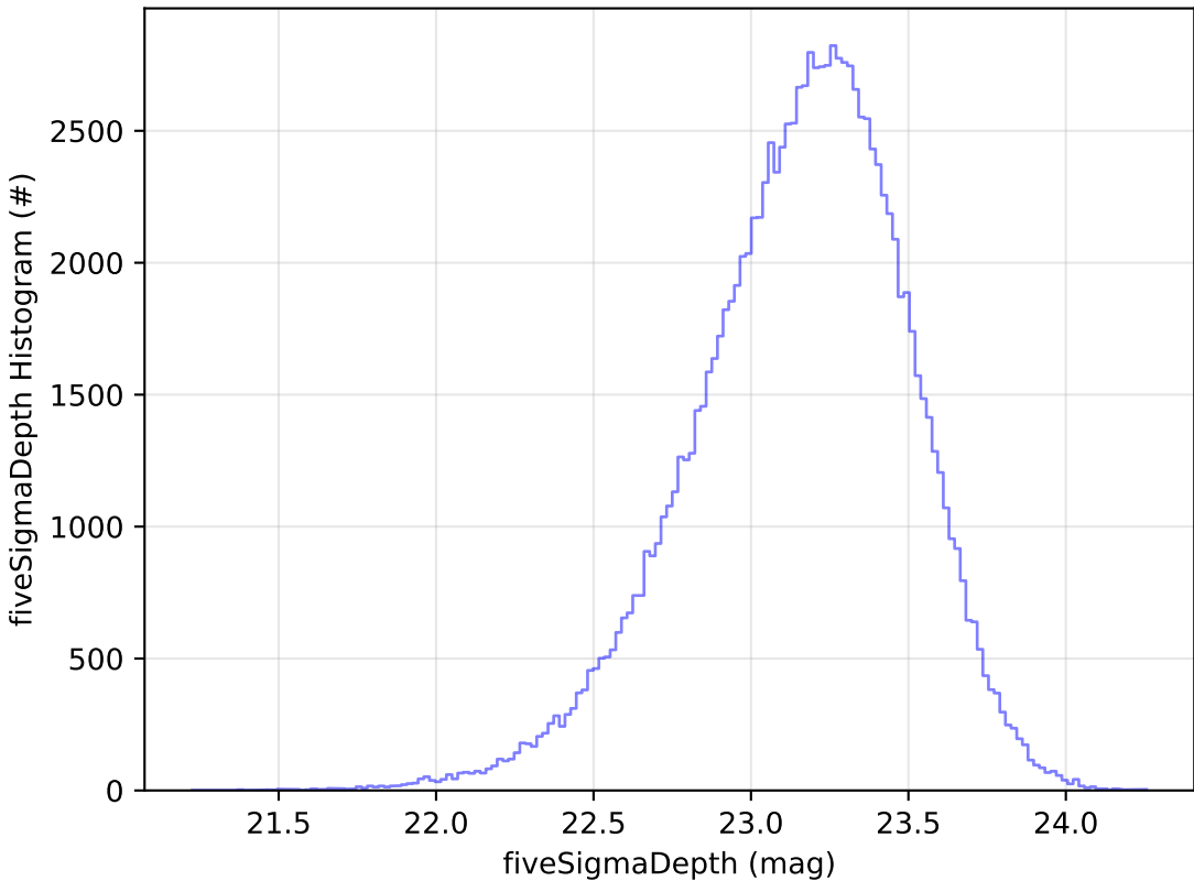
ddf_acor_sf20_lsf40_lsr10_v3.4_10yrs u: fiveSigmaDepth Histogram
