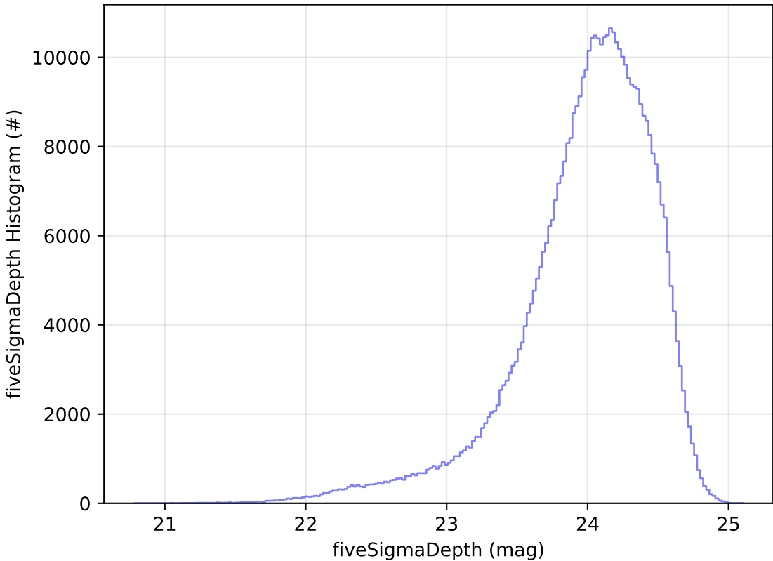
ddf_acor_sf20_lsf40_lsr10_v3.4_10yrs r: fiveSigmaDepth Histogram
