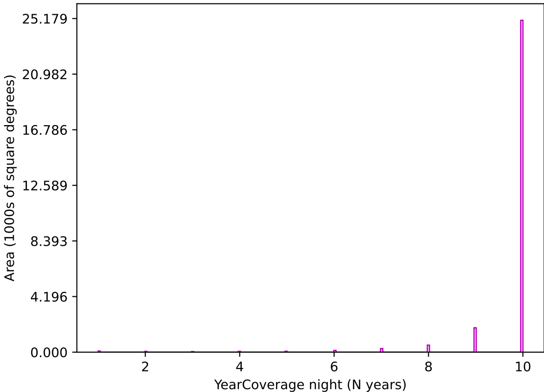
ddf_acor_sf20_lsf40_lsr10_v3.4_10yrs z band: YearCoverage night
