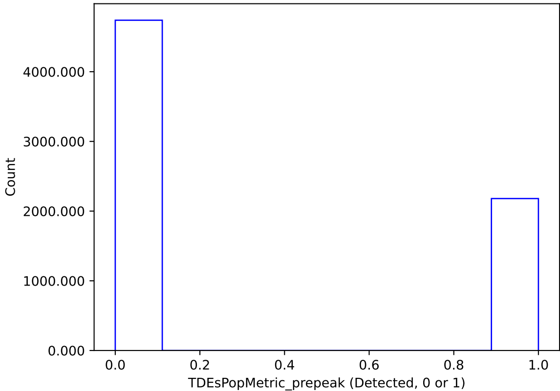
ddf_acor_sf20_lsf40_lsr10_v3.4_10yrs : TDEsPopMetric_prepeak
