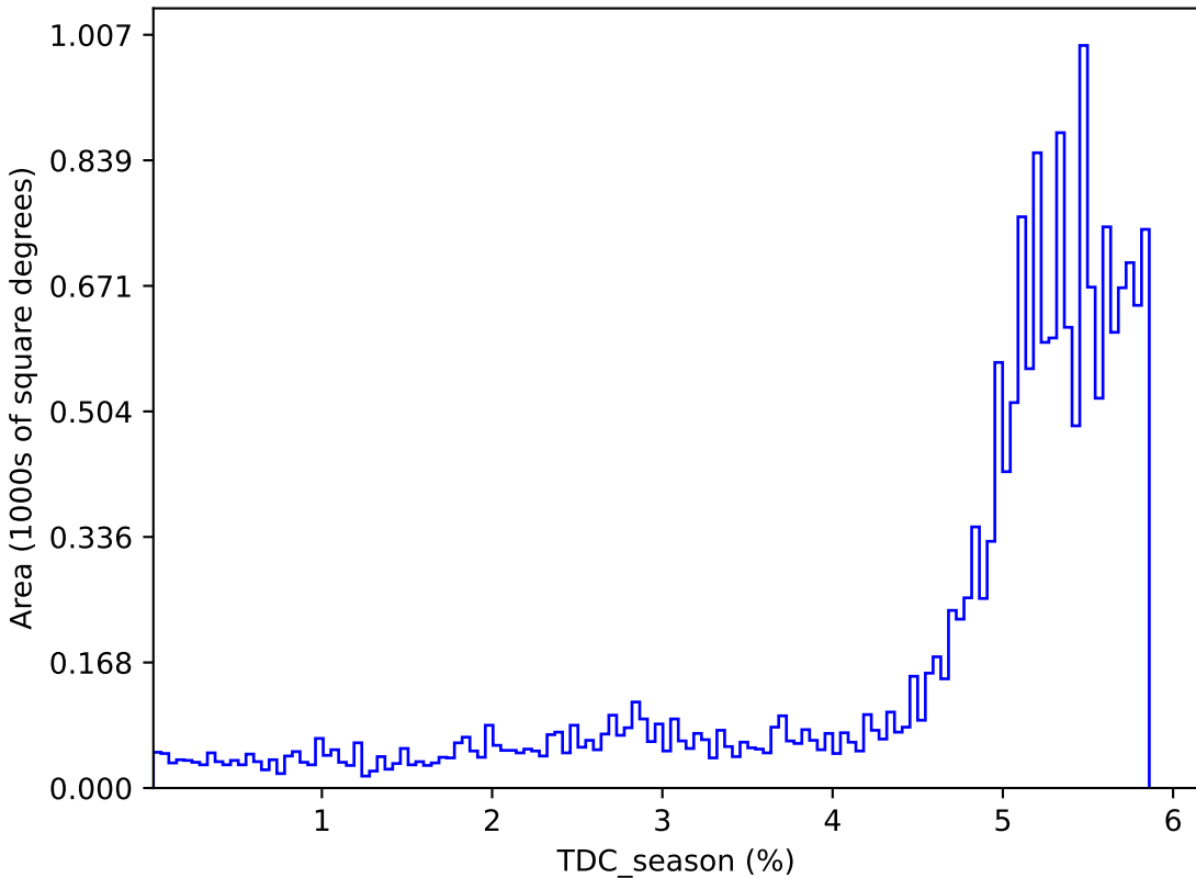
ddf_acor_sf20_lsf40_lsr10_v3.4_10yrs : TDC_season
