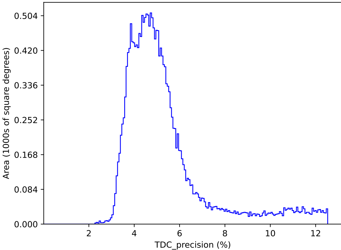
ddf_acor_sf20_lsf40_lsr10_v3.4_10yrs : TDC_precision
