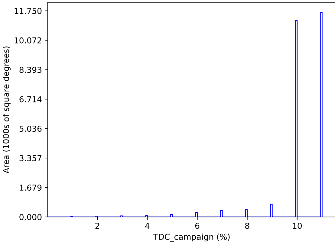
ddf_acor_sf20_lsf40_lsr10_v3.4_10yrs : TDC_campaign
