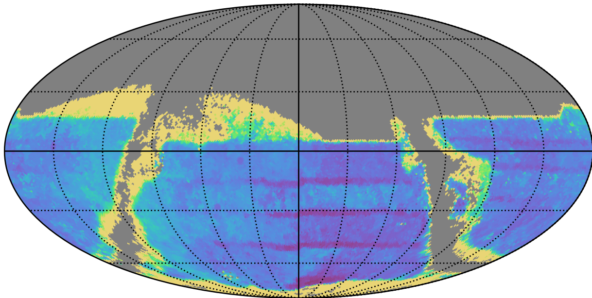
ddf_acor_sf20_lsf40_lsr10_v3.4_10yrs : TDC_accuracy
