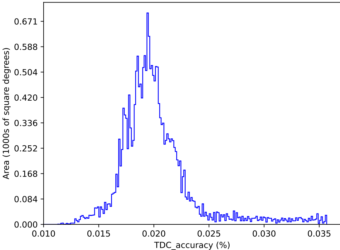
ddf_acor_sf20_lsf40_lsr10_v3.4_10yrs : TDC_accuracy
