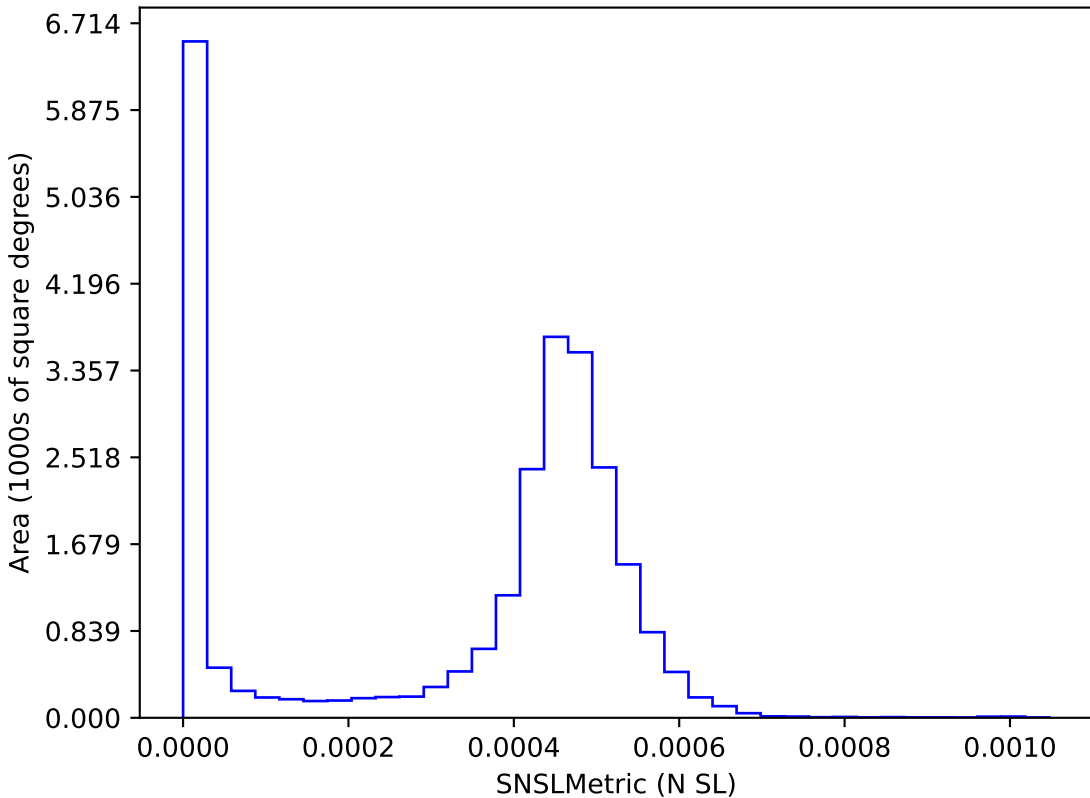
ddf_acor_sf20_lsf40_lsr10_v3.4_10yrs : SNSLMetric
