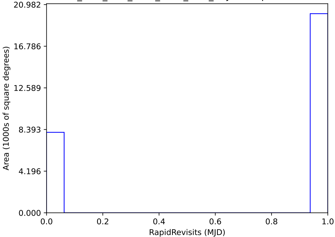
ddf_acor_sf20_lsf40_lsr10_v3.4_10yrs : RapidRevisits
