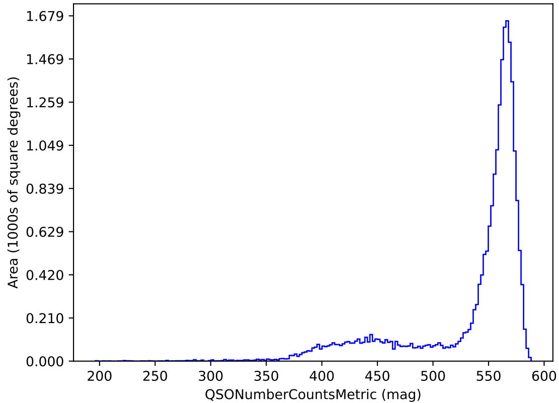
ddf_acor_sf20_lsf40_lsr10_v3.4_10yrs y band and non-DD: QSONumberCountsMetric
