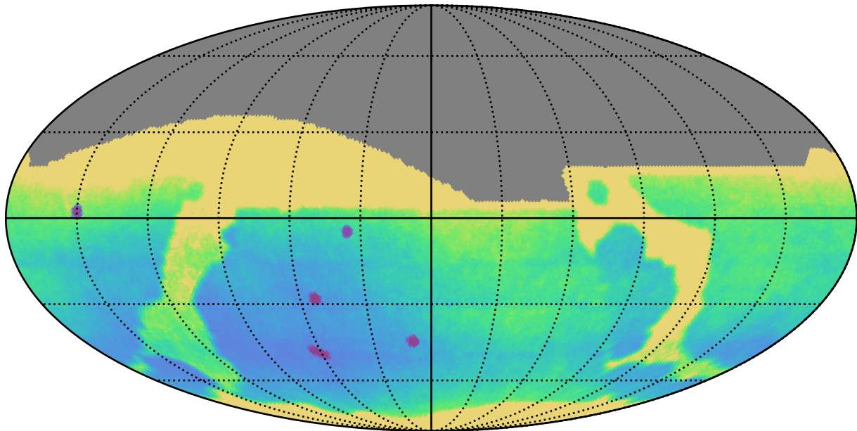
ddf_acor_sf20_lsf40_lsr10_v3.4_10yrs : Parallax Uncert @ 24.0
