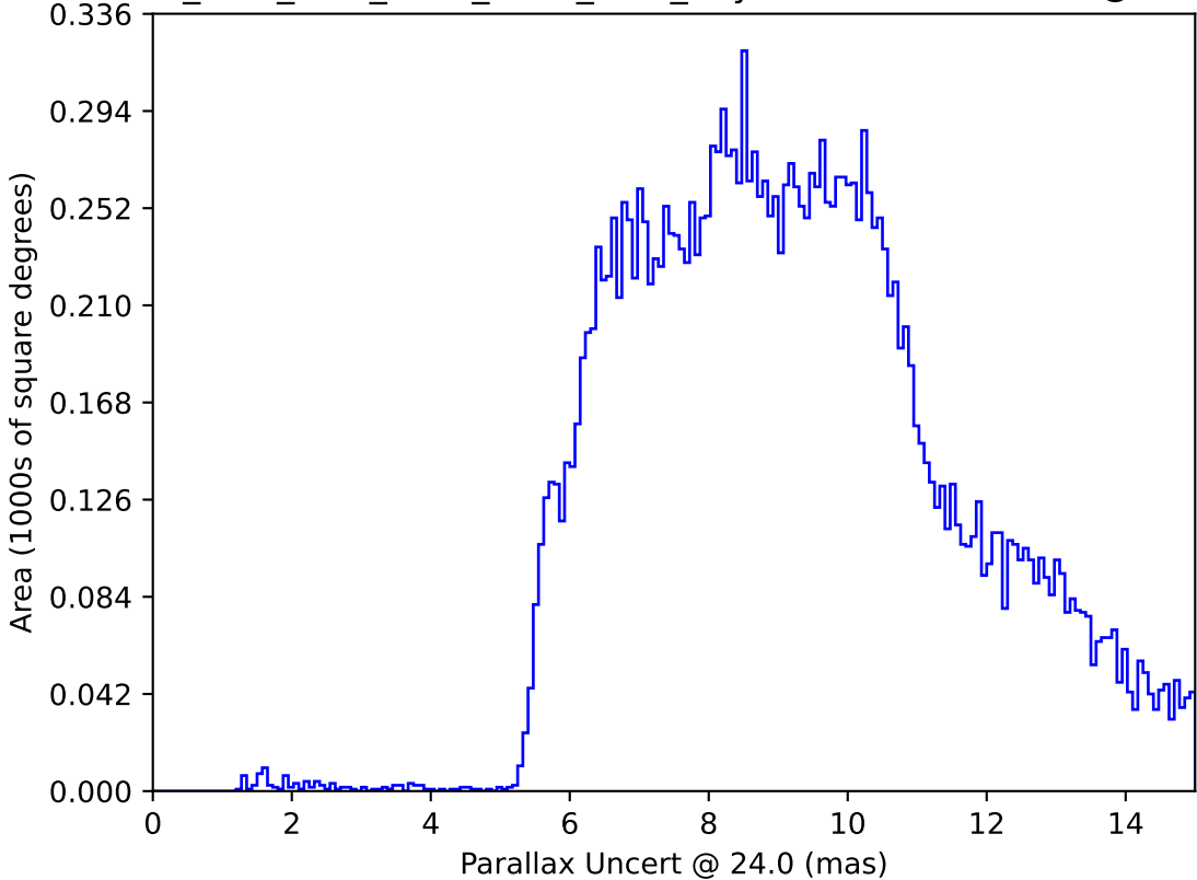
ddf_acor_sf20_lsf40_lsr10_v3.4_10yrs : Parallax Uncert @ 24.0
