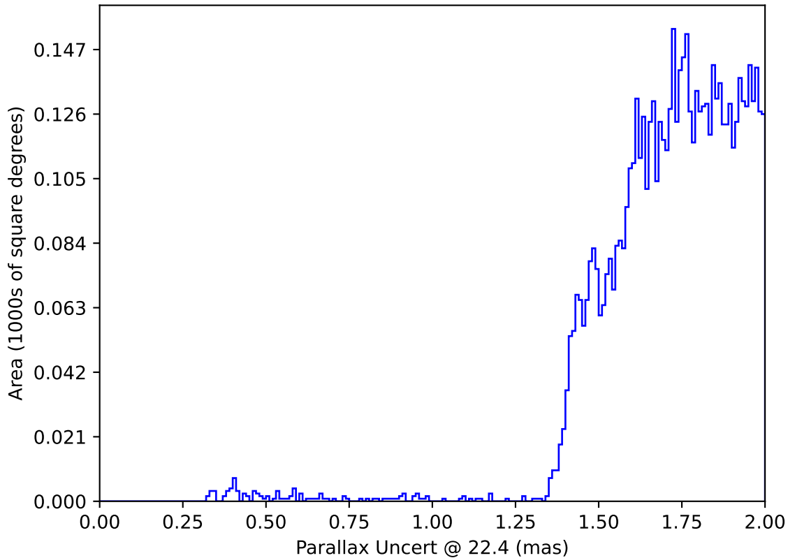
ddf_acor_sf20_lsf40_lsr10_v3.4_10yrs : Parallax Uncert @ 22.4
