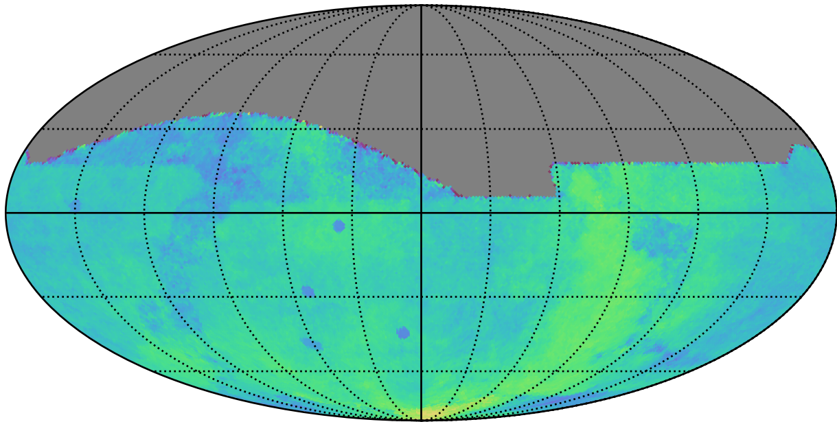
ddf_acor_sf20_lsf40_lsr10_v3.4_10yrs : Parallax Coverage @ 24.0
