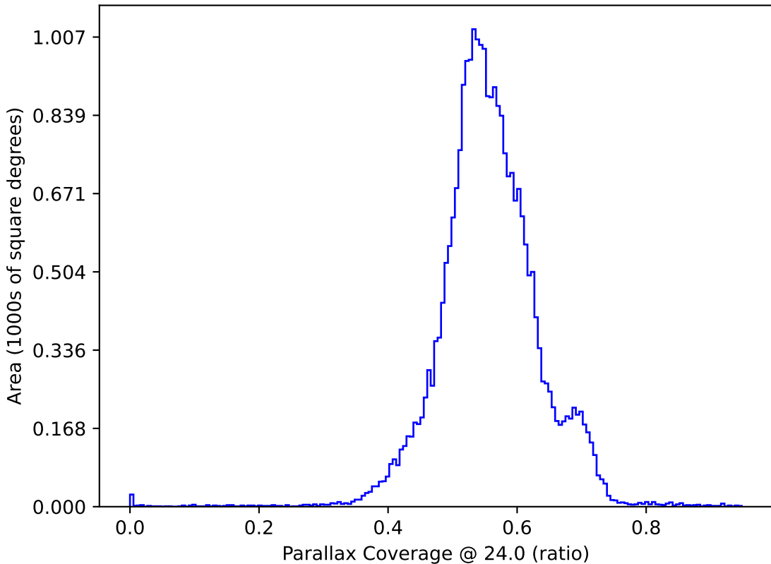
ddf_acor_sf20_lsf40_lsr10_v3.4_10yrs : Parallax Coverage @ 24.0
